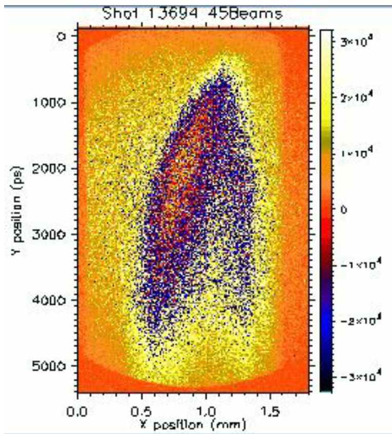
Figure 4.8: Streak camera record of emission.
