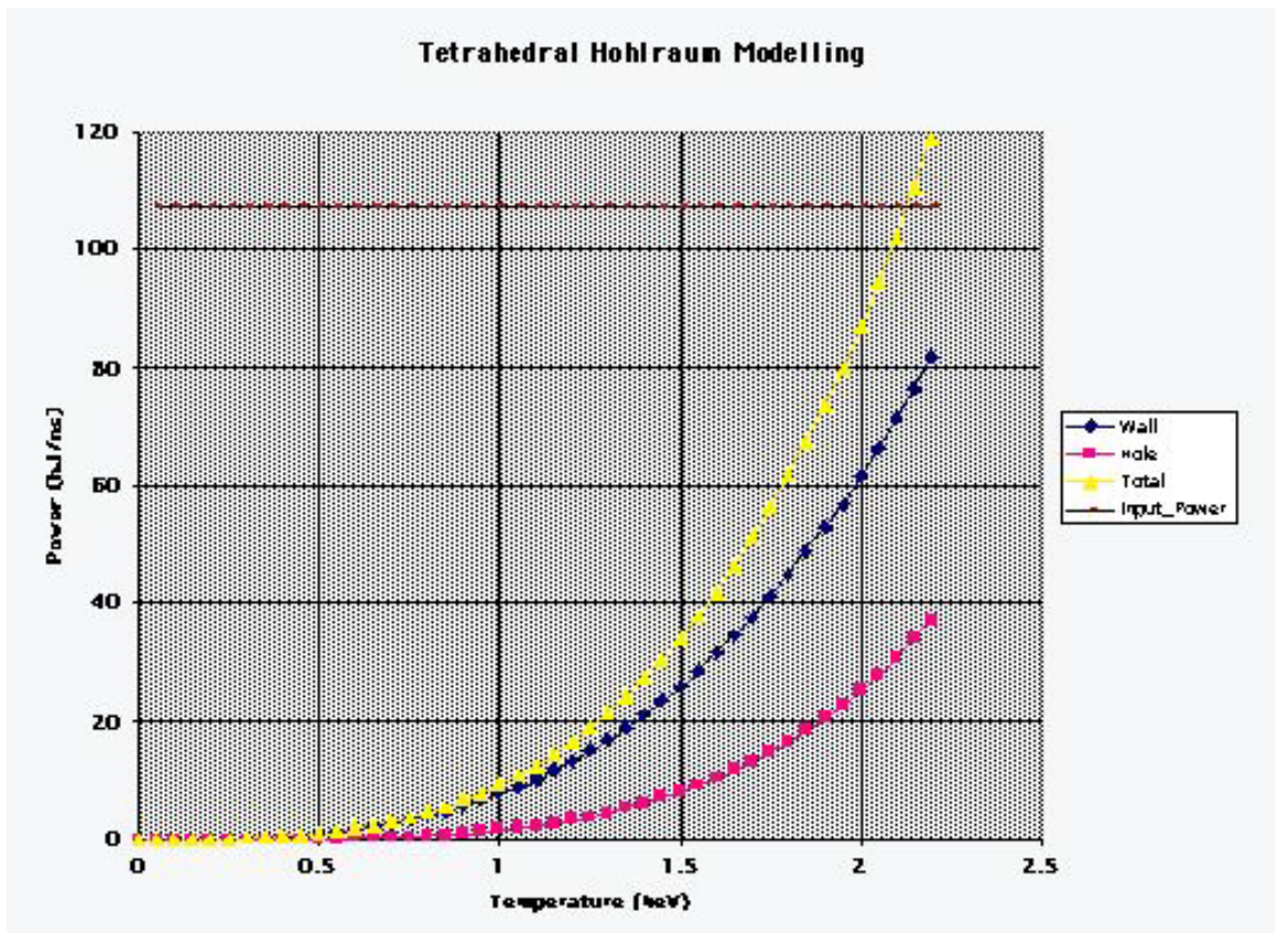
Figure 4.3: Hohlraum temperature vs temperature for 21.5 kJ incident and 90% absorption.
